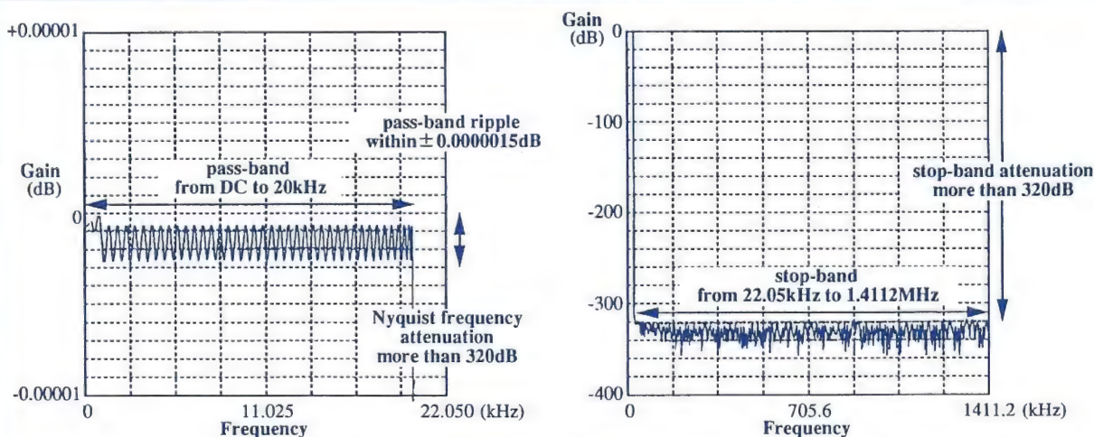
The characteristics and specifications of single stage 32767 taps and 64-bit coefficient FIR filter
